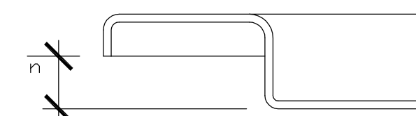
FIGURE 1: UNDERSIDE OF PAN TO TOPPLATE LIP
