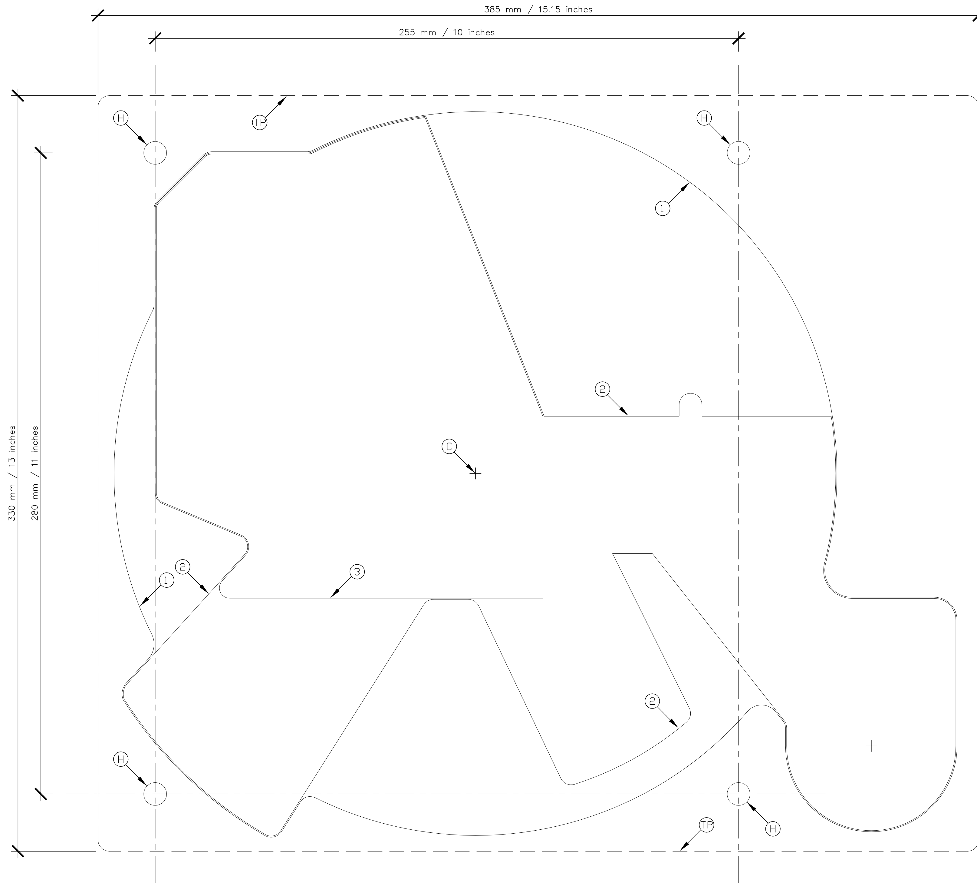
FIGURE 1: UNDERSIDE OF PAN TO TOPPLATE LIP
